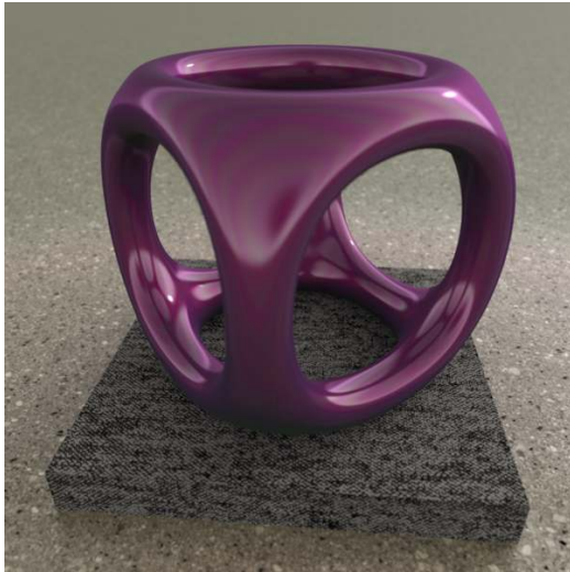
Fig. 5.14 - measured_bsdf
