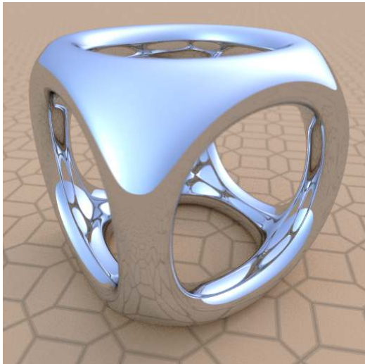
Fig. 5.3 - specular_bsdf
